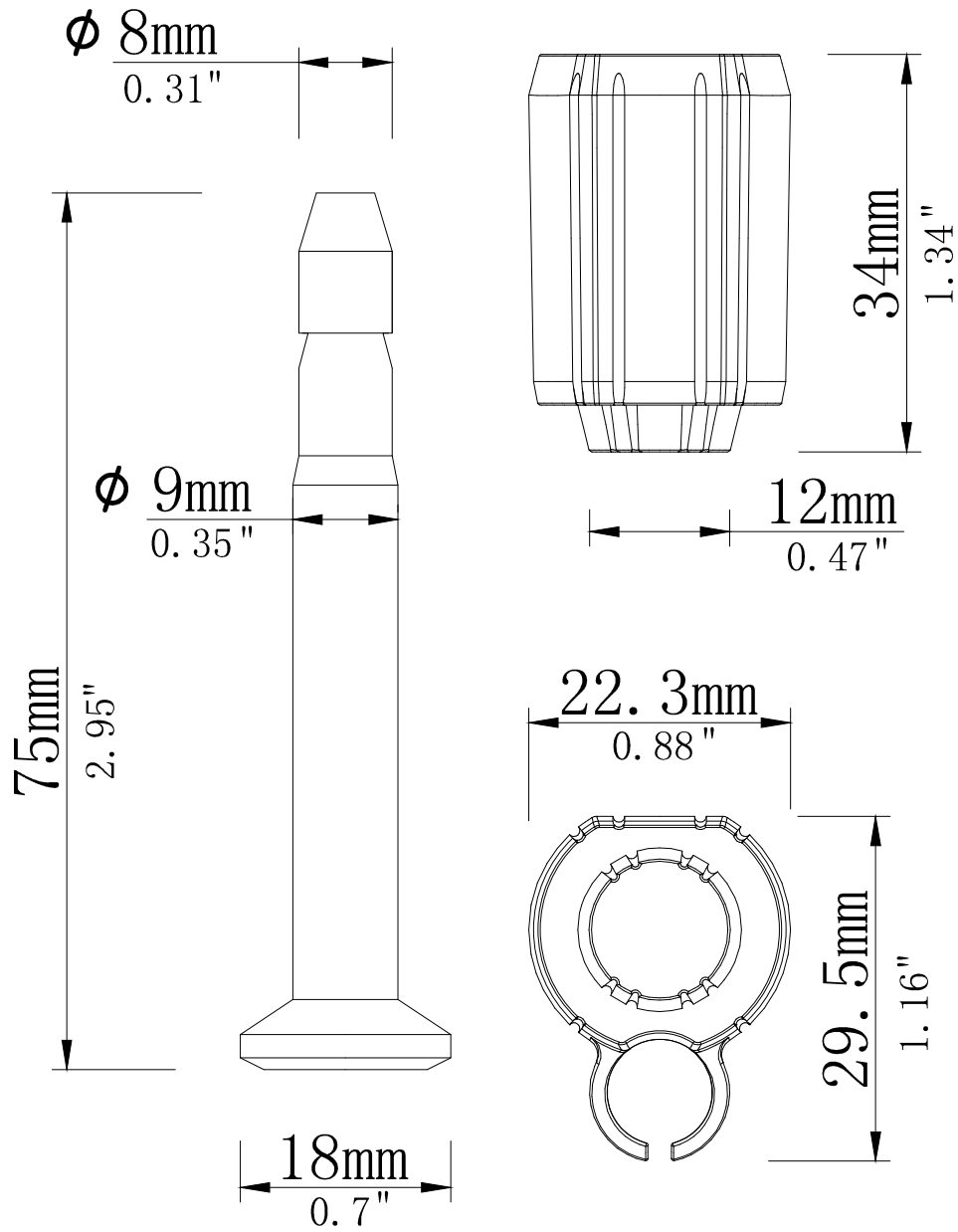
Model : GC-B003
